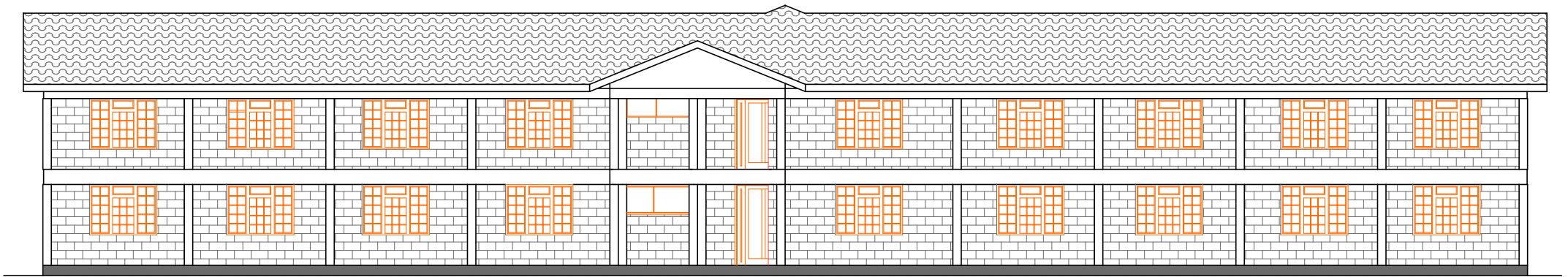
FRONT ELEVATION E-01
