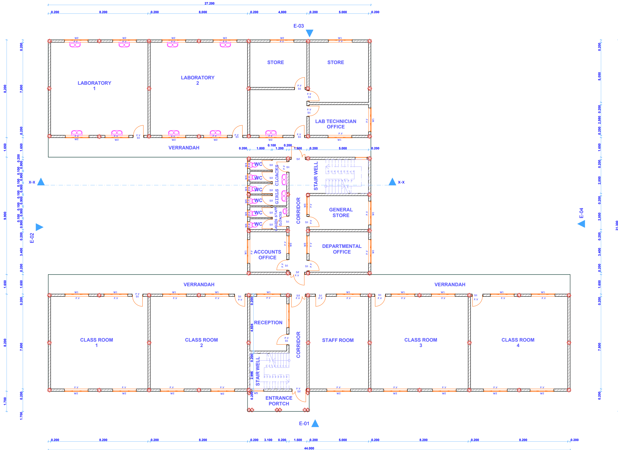
GROUND FLOOR PLAN LAYOUT
