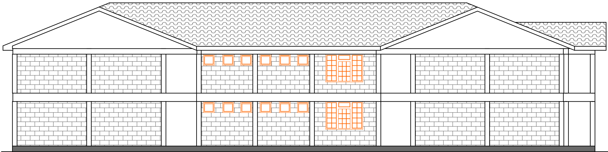
SIDE ELEVATION E-02
